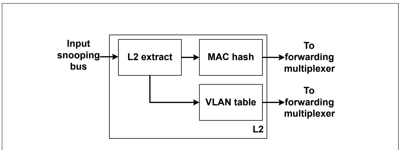
Figure 31.91 Block diagram of Layer 2 forwarding
