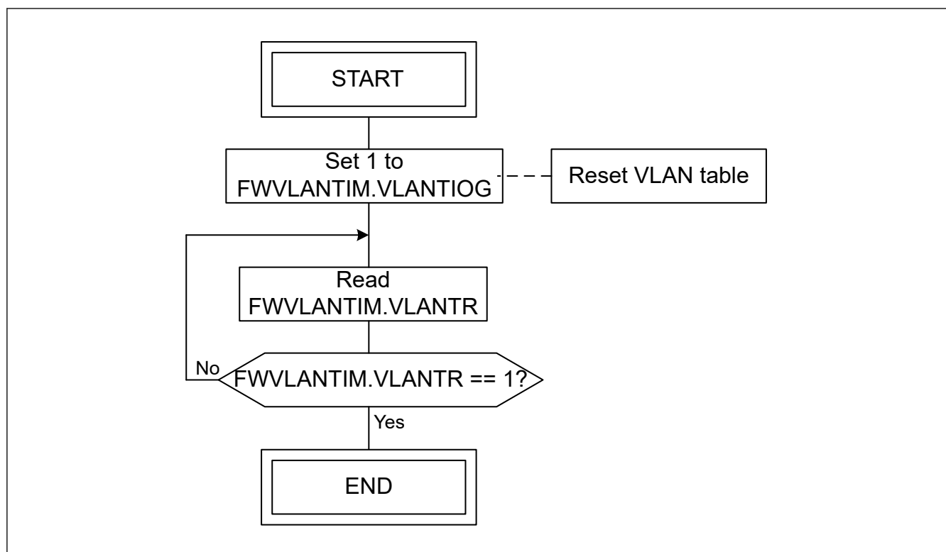
Figure 31.16 Reset flow of VLAN table
