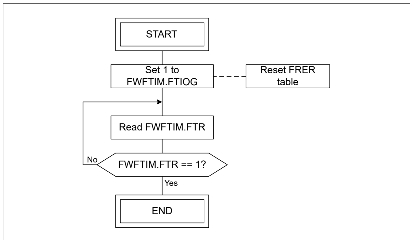
Figure 31.30 Reset flow of FRER table
