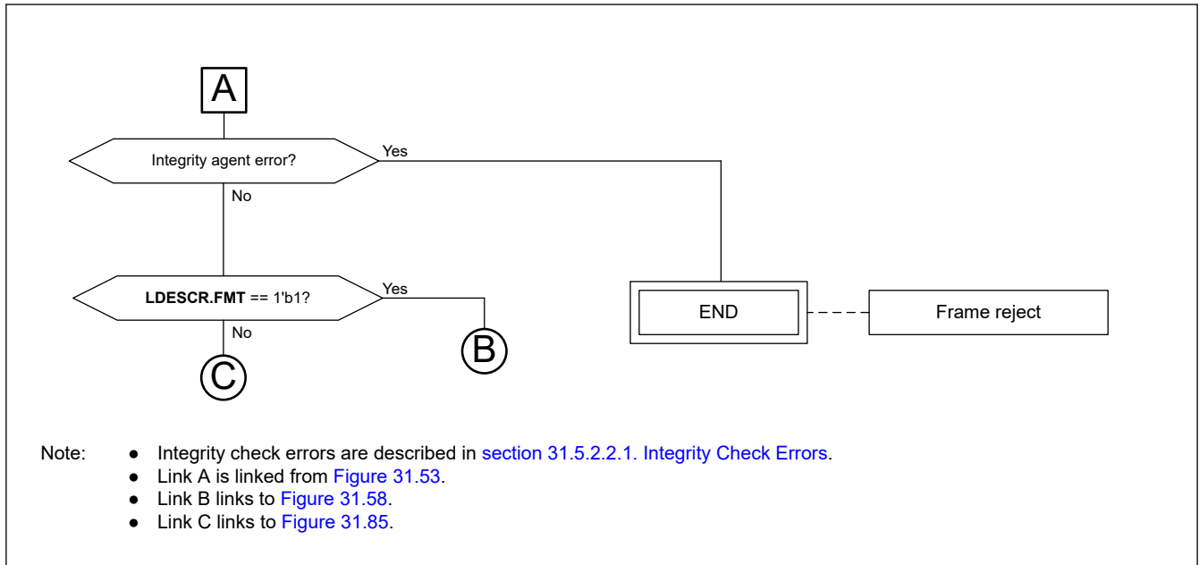
Figure 31.56 Integrity check flow
