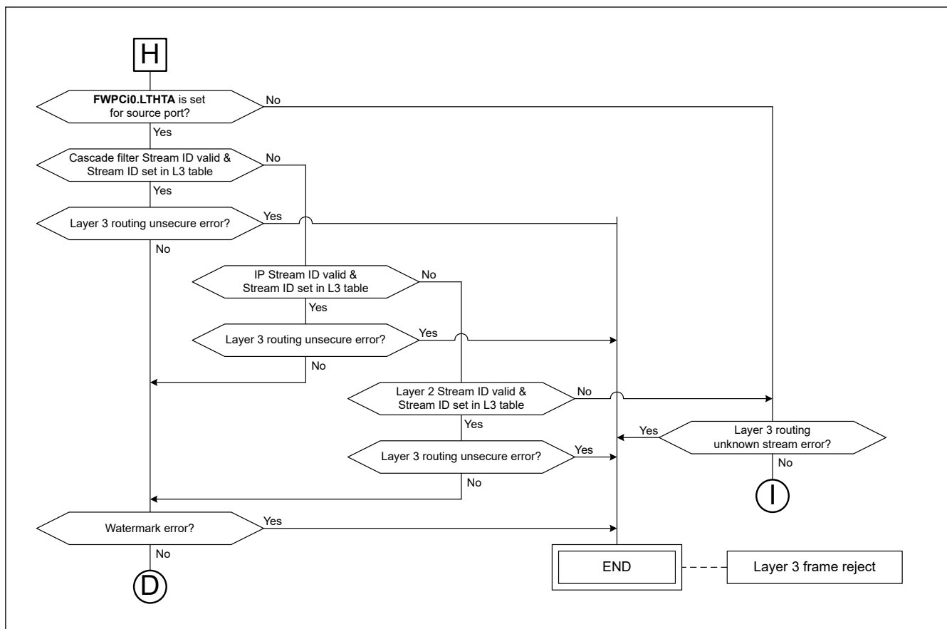
Figure 31.86 Layer 3 forwarding/routing unsecure flow
